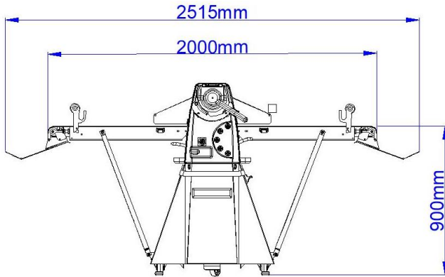
VISTA FRONTAL 1
